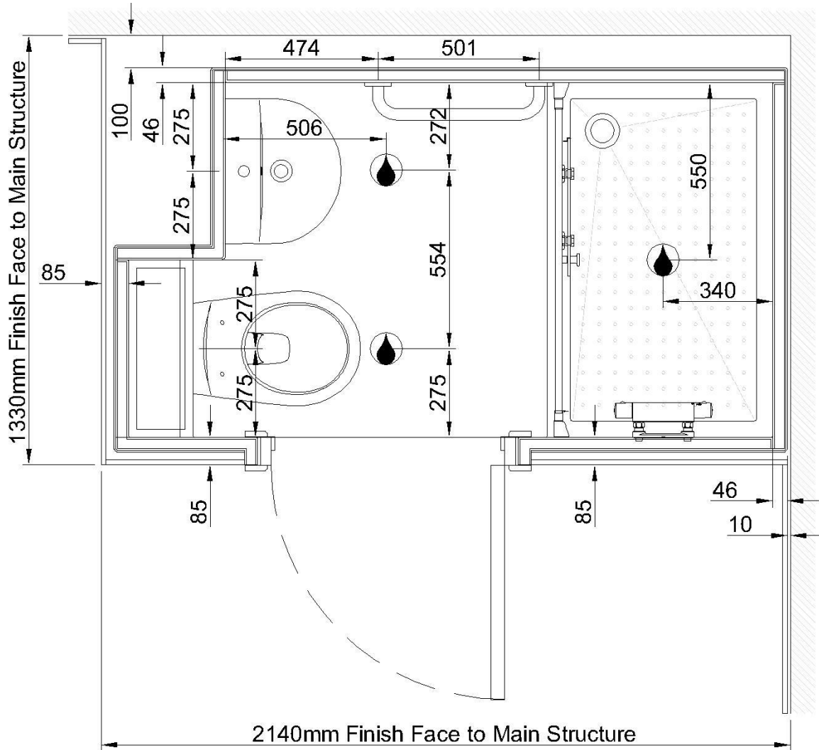
Floor Plan
